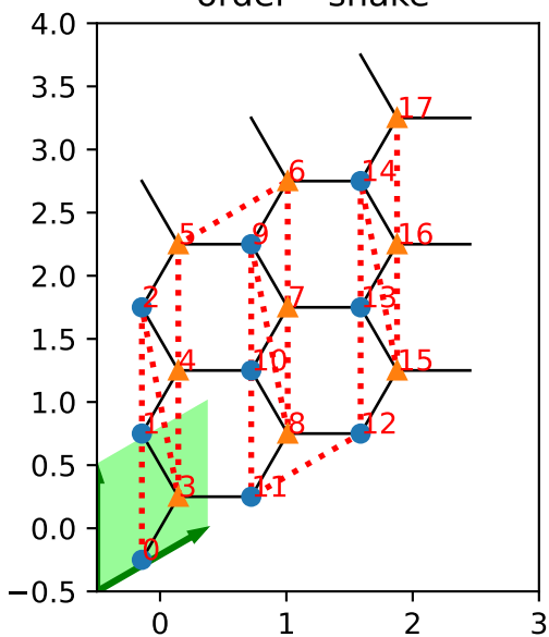
order='snake'
