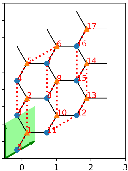
order='snakeCstyle'
