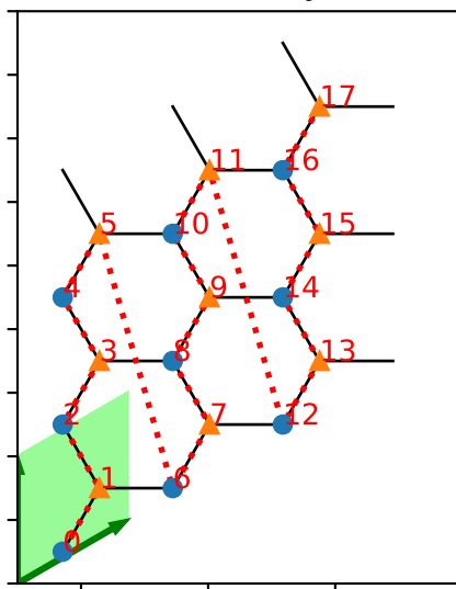
order='Cstyle'
