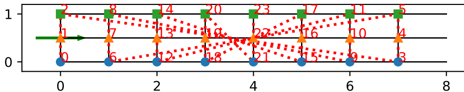
order='folded'
