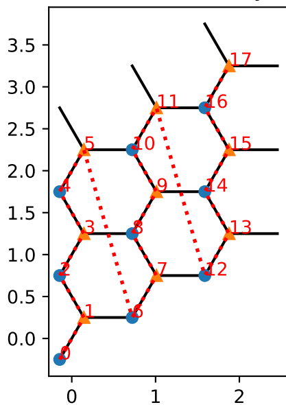
order = "order='Cstyle'"
