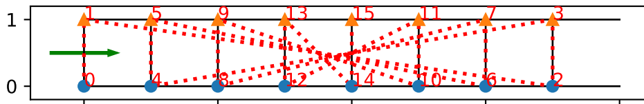
order='folded'
