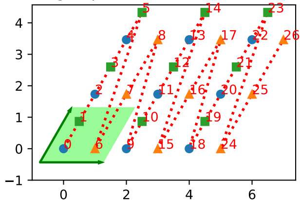
("grouped", [(0, 2), (1,)], None)
