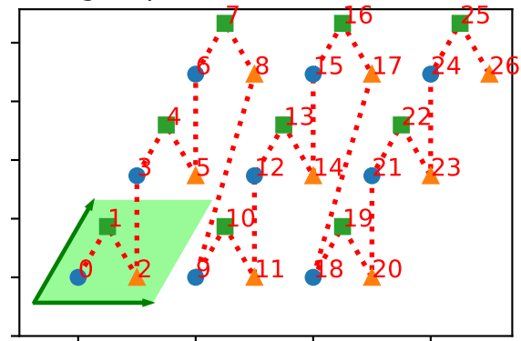
("grouped", [(0, 2, 1)], None)
