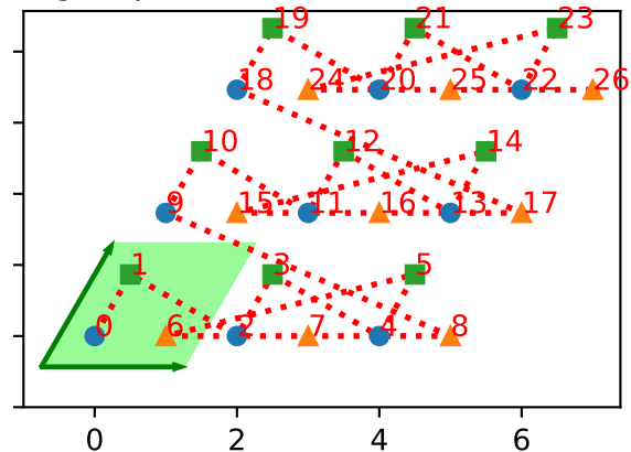
("grouped", [(0, 2), (1,)], [1, 0, 2])
