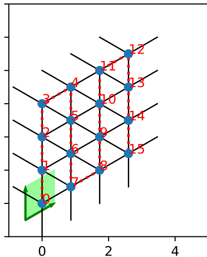
order='snake'
