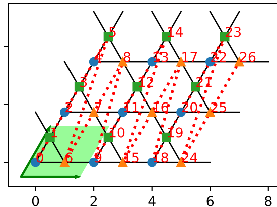
order='rings'
